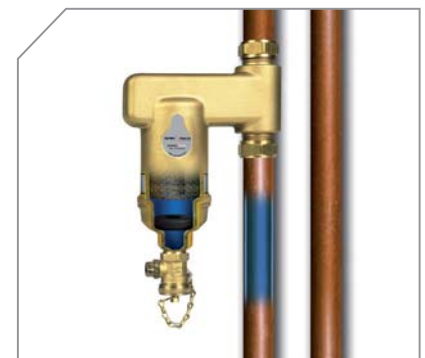
▶ 3: Continuous Dirt Separation
