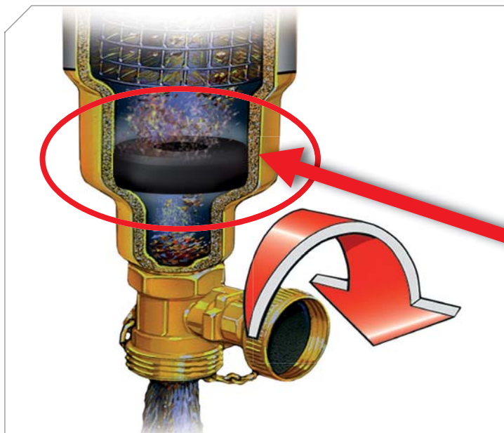
▷ Dirt Separator with self cleaning magnet inside
